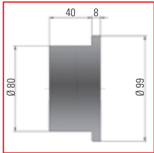
ADJUSTABLE STANDARD WHEELS
